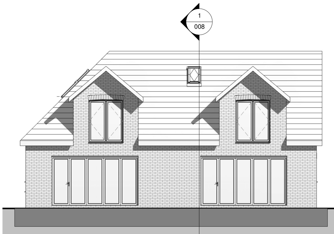
Rear Elevation
